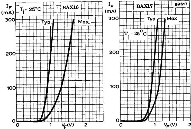
FORWARD CHARACTERISTICS
