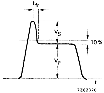
Fig. 4 Waveform.
