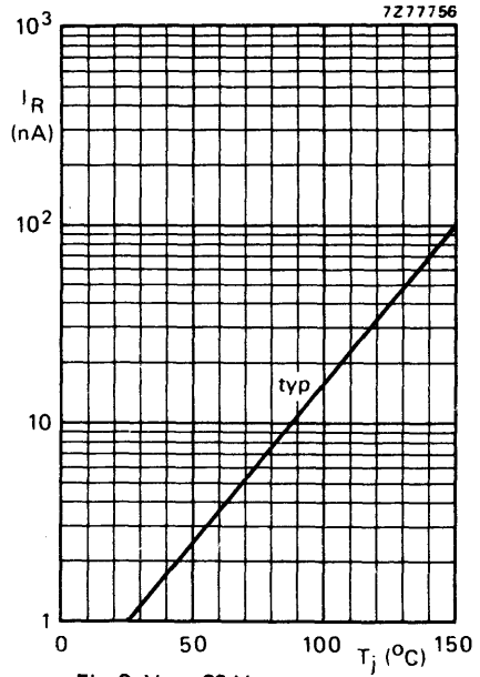
Fig. 3 V_R = 20 V.
