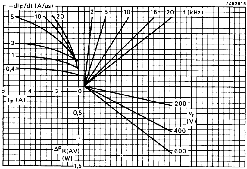
Fig. 9 Nomogram: power loss ( \Delta P_R(AV) ) due to switching only. To be added to steady state power losses (see also Fig. 4).
