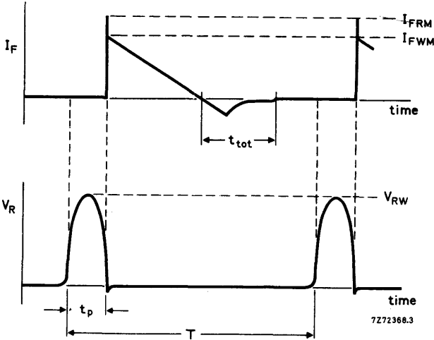
Fig. 7 Basic waveforms.
