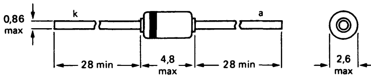
Fig. 1 DO-41 (SOD-66).
