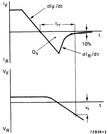
Fig. 4 Definitions.
