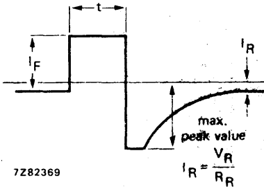
Fig. 3 Output waveform.
