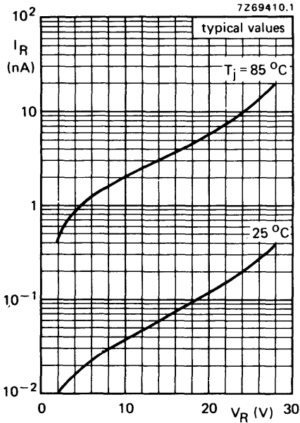
Fig. 2 Typical values.
