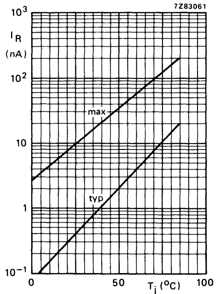
Fig. 5 V_R = 28 V.
